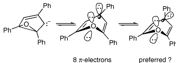
Figure 3. Possible conformations and valence isomerization of a pyranil anion
