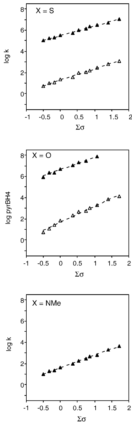
Figure 5. Plots of logarithms of second-order rate constants for reduction by sodium cyanoborohydride (Δ) or sodium borohydride (▲) against Hammett substituent constants of heteroaromatic cations with X = S, O, or NMe
