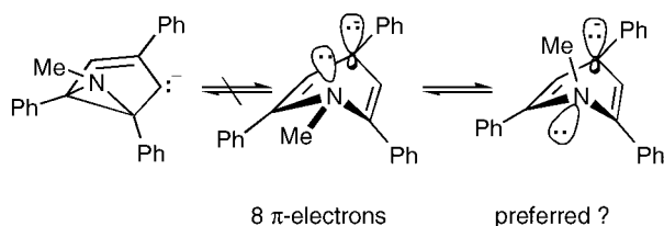
Figure 4. Possible conformations and valence isomerisation of a pyridyl anion
