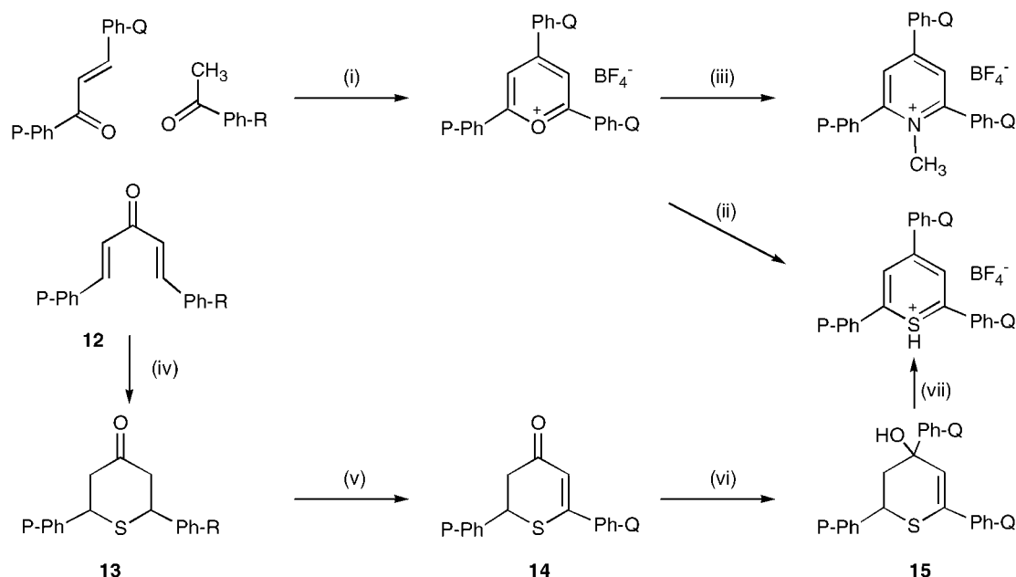
Scheme 1. Preparation of heterocyclic cations. Reagents: - (i) see text; (ii) Na 2 S then HBF 4 ; (iii) MeNH 3 then HBF 4 ; (iv) H 2 S/NaOAc; (v) NCS/pyridine; (vi) Q-PhLi in THF; (vii) HBF 4 , Ph 3 COH
